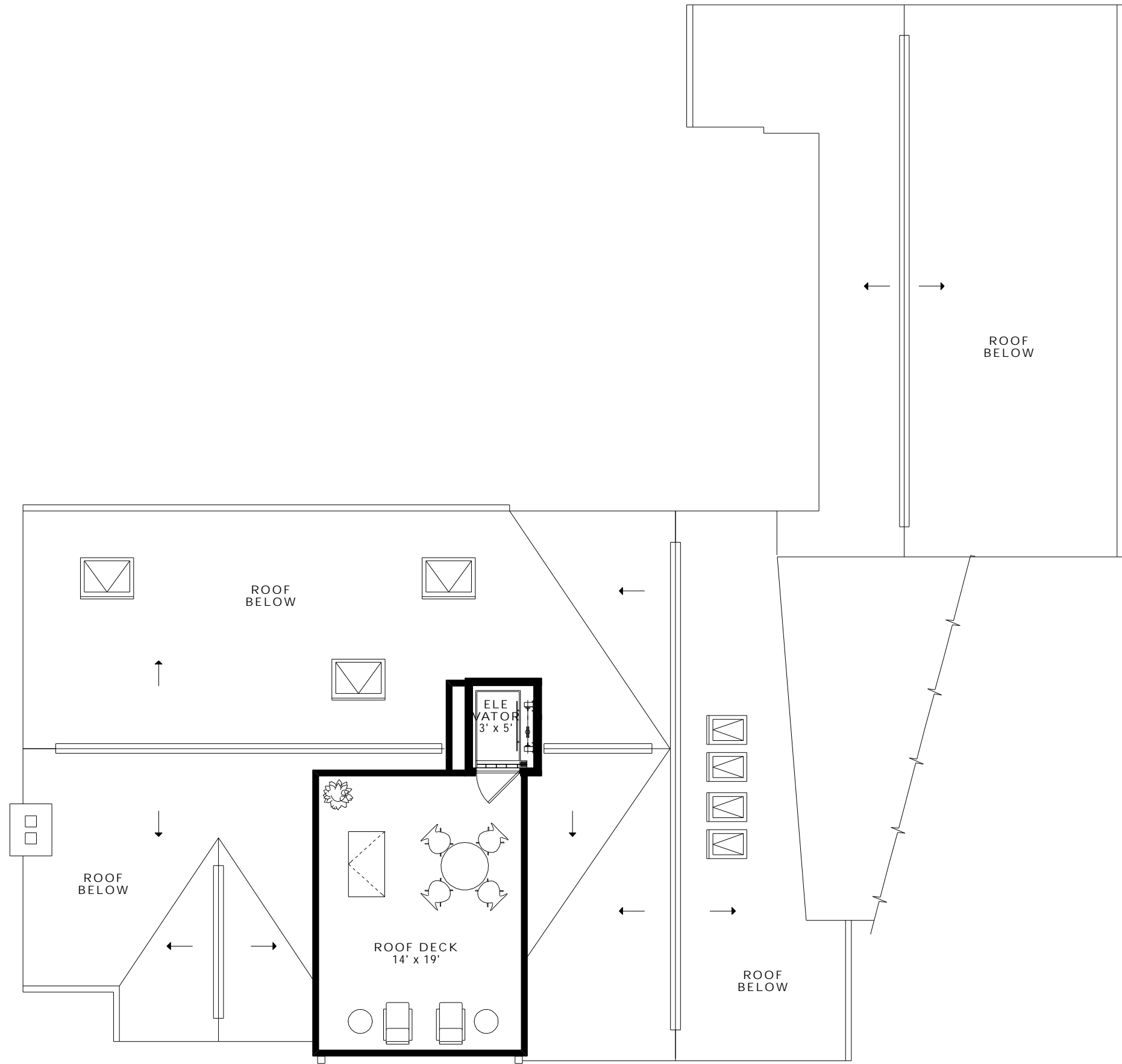
ROOF DECK (ALL SIZES APPROXIMATE)
